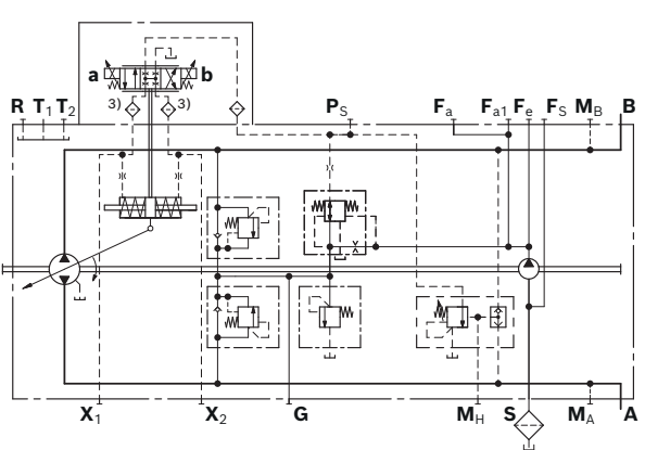
▼ Circuit diagram, version with DA control valve 2)
