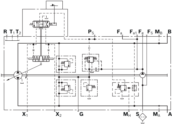
Circuit diagram, version with DA control valve and neutral position switch 1)
