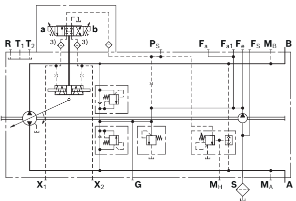
▼ Circuit diagram, standard version 2)
