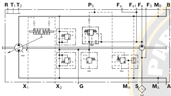
▼ Circuit diagram, version with DA control valve 1)
