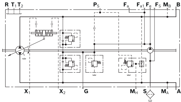
▼ Circuit diagram, standard version 1)
